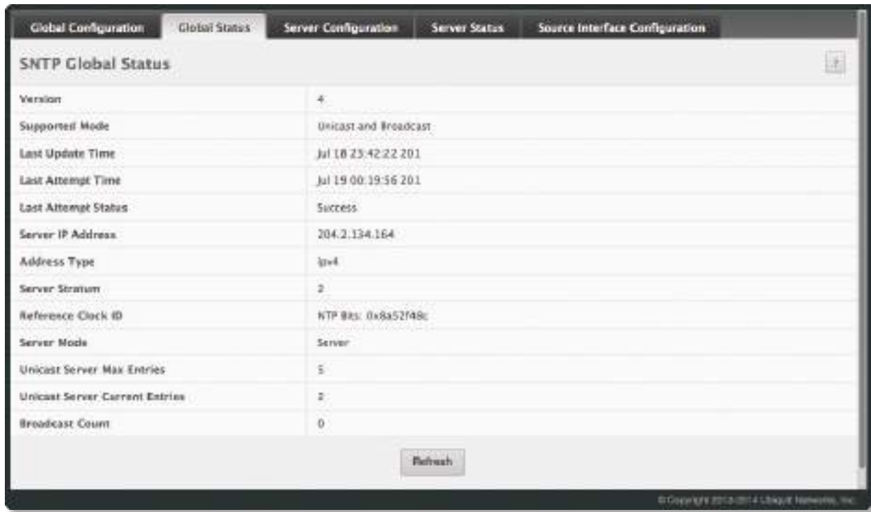
SNTP Global Status
