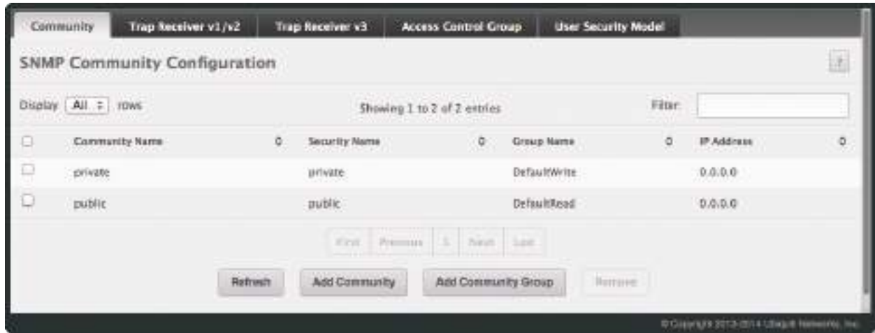
SNMP Community Configuration
