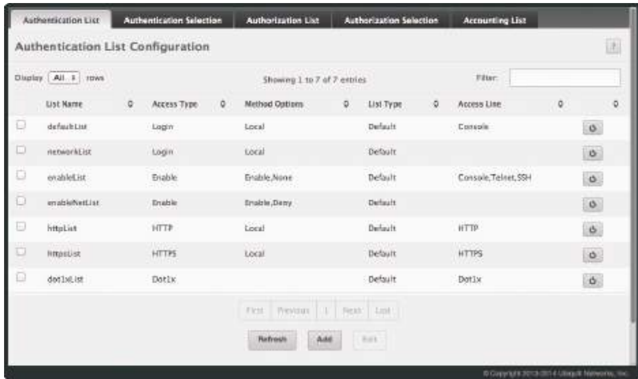
Authentication List Configuration
