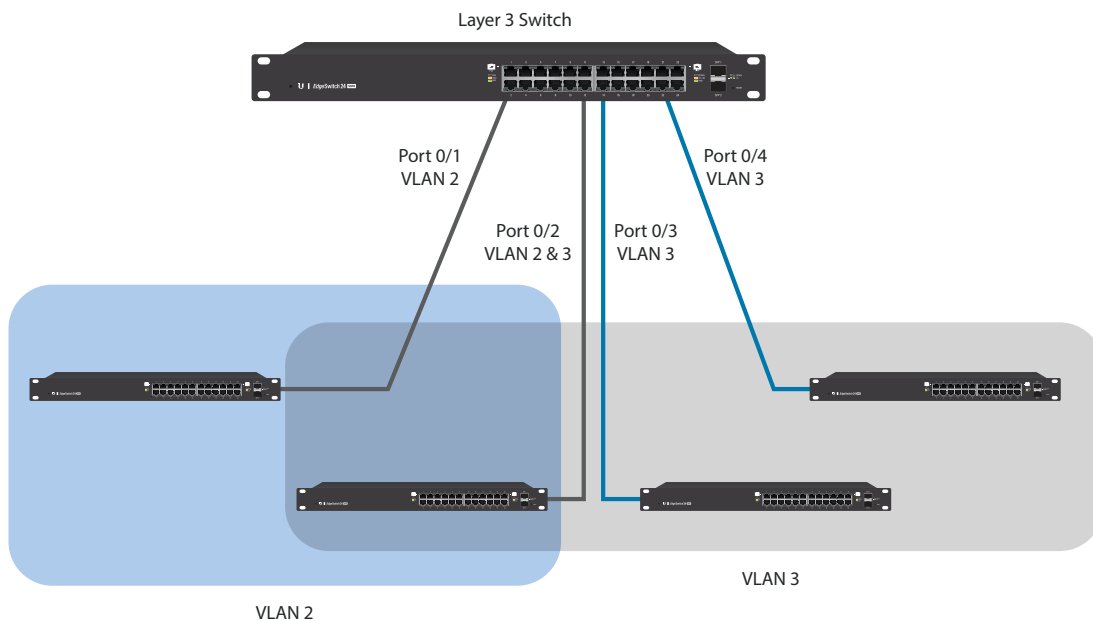
VLAN Example Network Diagram
