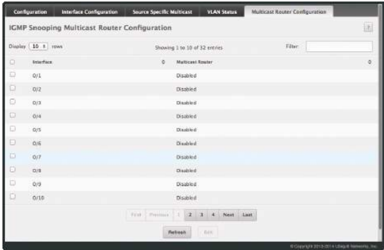
IGMP Snooping Multicast Router Configuration
