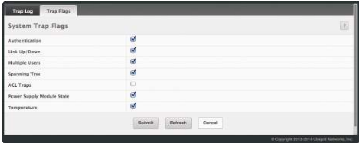
System Trap Flags
