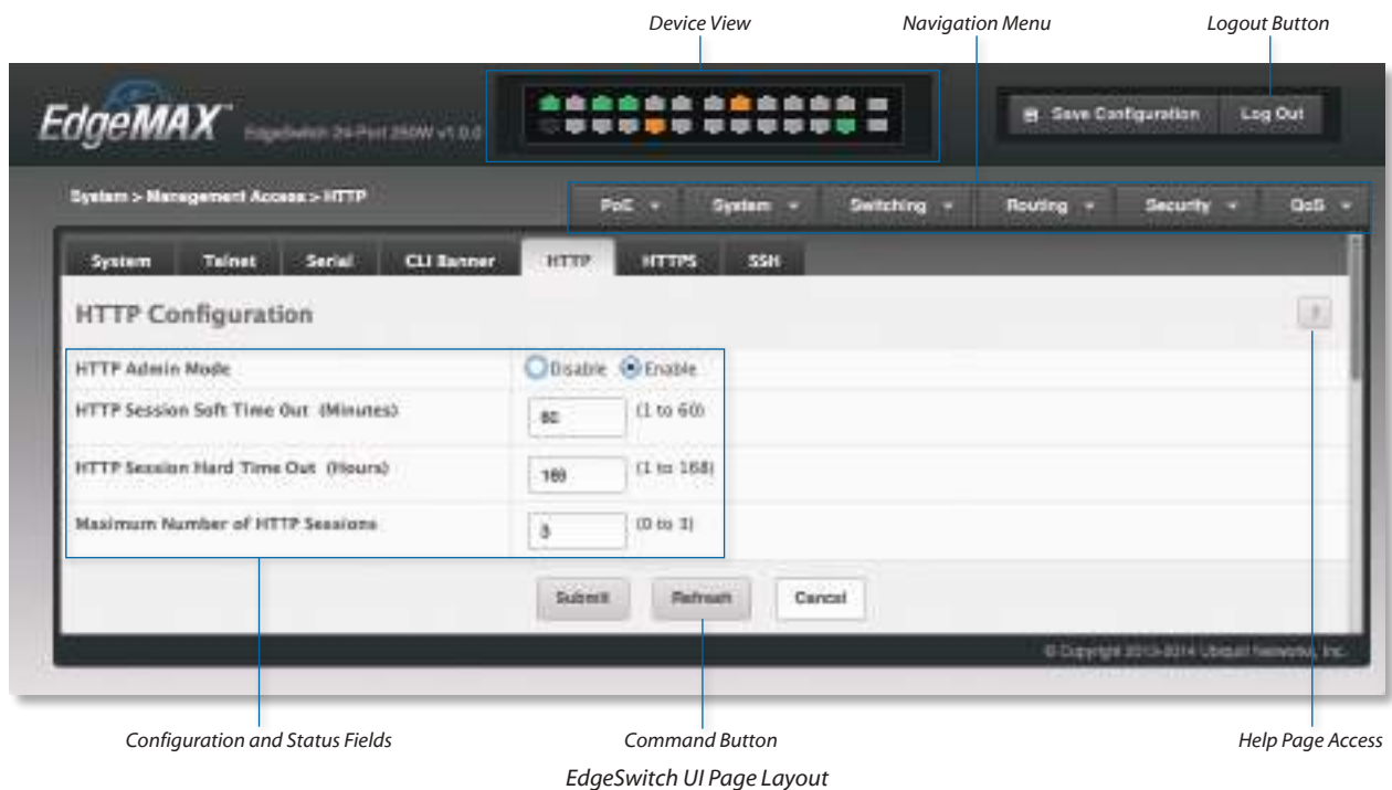
EdgeSwitch UI Page Layout
